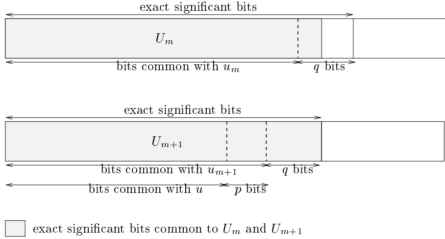
Figure 1: significant bits of U_m and U_{m+1}
