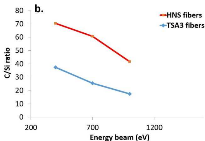
Figure 4. Overview spectra of the surface of the HNS and TSA3 desized fibers at 700 eV (a.) and C/Si ratio of the HNS and TSA3 desized fibers relative to the energy beam (b.)
