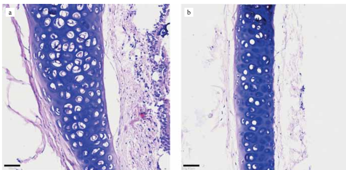
Fig. 1. Tracheal cartilage sample after devitalization: a – native tracheal tissue; b – devitalized tracheal scaffold. Hematoxylin-eosin staining. The scale bar is 50 µm. \times 100
