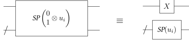
Figure 8: Desentangling one qubit in state preparation
