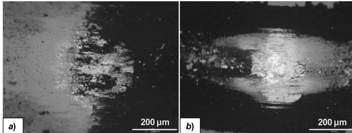
Figure 14. Wear scar of Al 2 O 3 corundum ball sliding against MoS 2 TiW coating manufactured on X38CrMoV5-1 steel: a) after the 450 meter test at 25 °C, b) after the 800 meter test at 200 °C.
