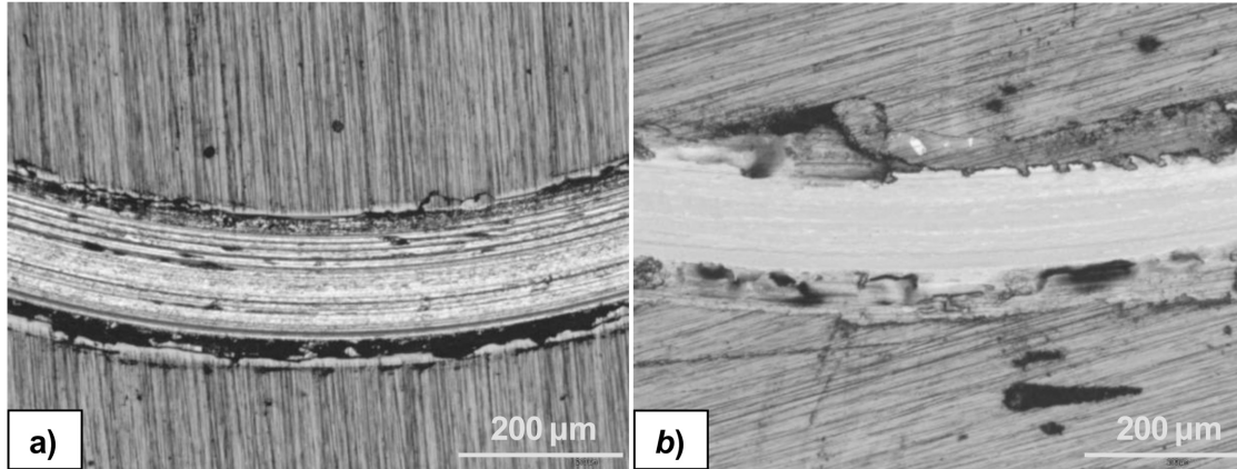
Figure 10. Wear tracks of MoS 2 TiW coating manufactured on X38CrMoV5-1 steel sliding against Al 2 O 3 ball: a) after the 450 meter test at 25 °C, b) after the 800 meter test at 200 °C.
