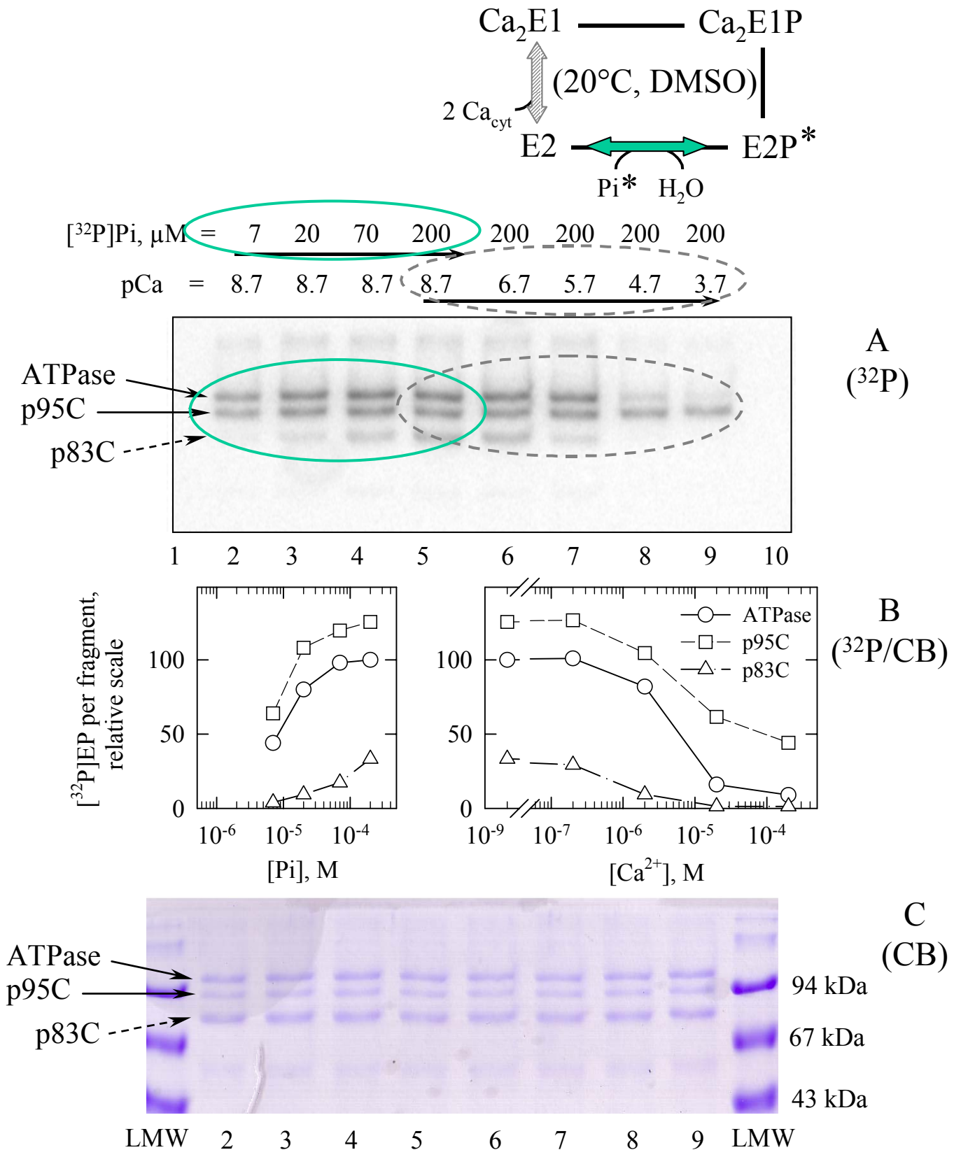
Fig 5. Equilibrium phosphorylation from [^{32}\text{P}]\text{Pi} of the p95C peptide occurs with quasi-normal affinity for Pi. Inhibition by \text{Ca}^{2+} is slightly less pronounced.
