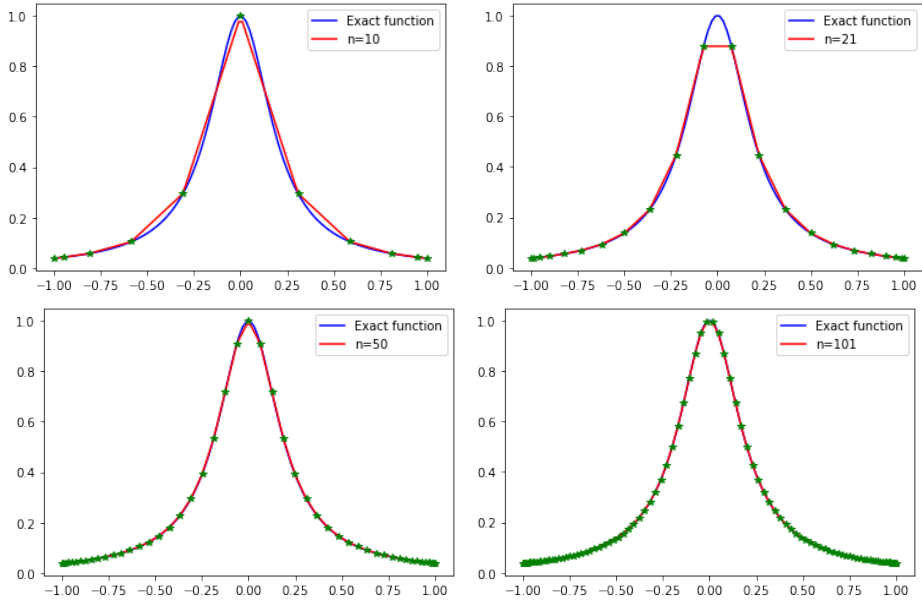
Figure 3: Relu interpolation with Chebychev points.
