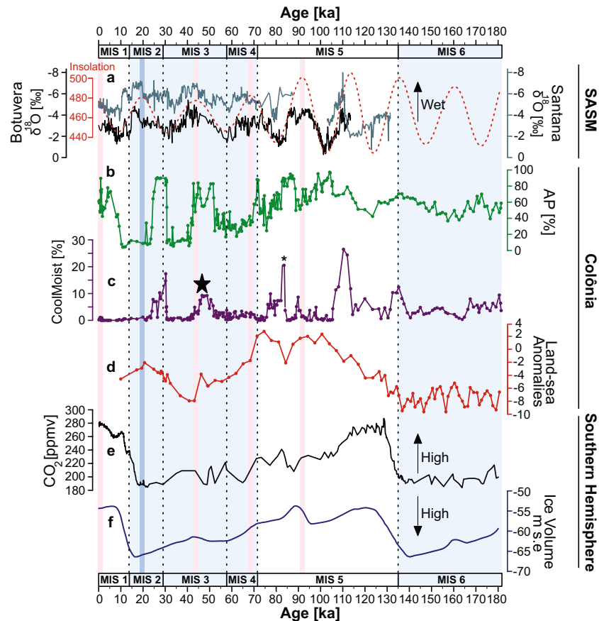
Figure 3. Regional comparison during the last 180 ka. (a) Speleothem records (Botuverá (black) and Santana (gray)) 9,42 plotted with insolation ( \text{W/m}^2 ) at latitude 23^{\circ}52'03''\text{S} using La2004 86 (red dashed line). (b) Arboreal pollen percentages (AP) from Colônia (CO3 and CO14). (c) Percentage curve of the sum of cool moist conifers Araucaria and Podocarpus ; the black star locates the last continuous occurrence of Araucaria , and asterisk represents ca. 60% of Podocarpus (see Methods section). (d) Land-sea temperature gradient. (e) p\text{CO}_2 (Lüthi et al. 89 ). (f) Total ice volume represented in m.s.e. (meters sea-level equivalent) for the Antarctic ice sheet 45 . The marine isotopic stage boundaries ages are based on the LR04 \delta^{18}\text{O} stack 38,87 . The boundary between MIS 5 and 6 is based on Henderson and Slowey 88 . Pink bands highlight the maximum insolation peaks of influence of the SASM system during the last 95 ka. The blue band also highlights the maximum insolation peak but emphasises the differences in Colônia's proxies compared with the regional datasets.
