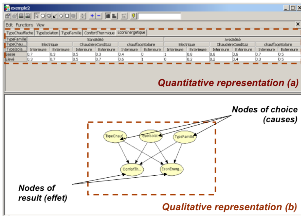
Figure 9. Implementation of a Bayesian network; (a) Filled Informations conditional probability tables; (b) Graphic description model. Bayesian network interface HUGIN [45].
