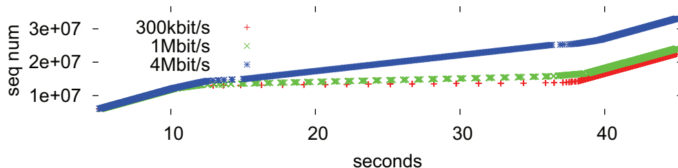
Figure 10. Handover scenario with various WWAN bandwidth and (10Mb/s, 10ms) WLAN.
