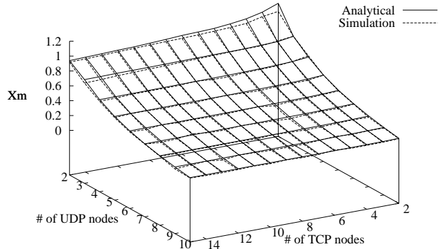
Figure 8: TCP/UDP scenario 1
