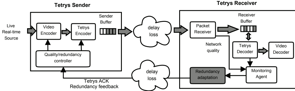
Figure 2: Adaptive Tetrays framework for real-time video transmission.
