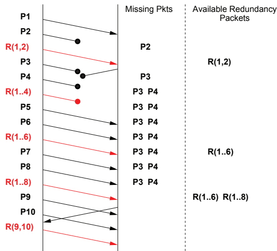
Figure 1: A simple data exchange with Tetrys ( k = 2 ) [9].
