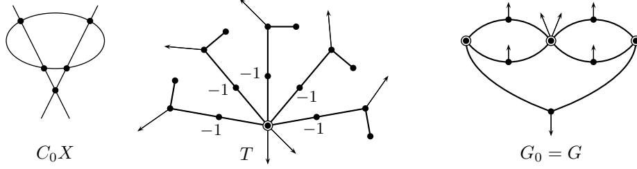
FIGURE 6. Example 4.4: A pair of lines intersecting an oval.
