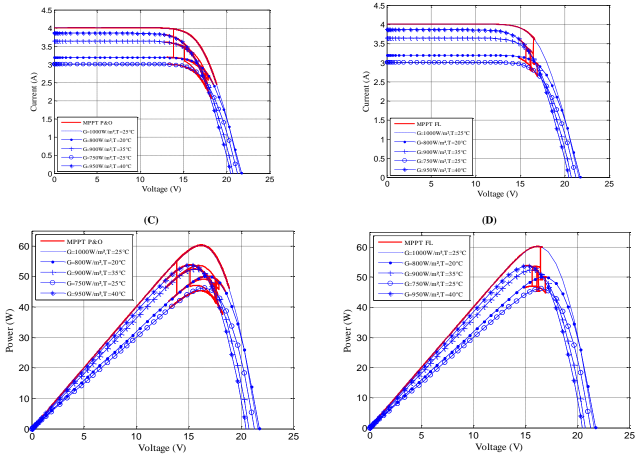
Fig. 9: Comparison of MPP Convergence of I-V and P-V Characteristics for Profile 1 Using MPPT Based on P&O (A) and (C) or FLC (B) and (D).
