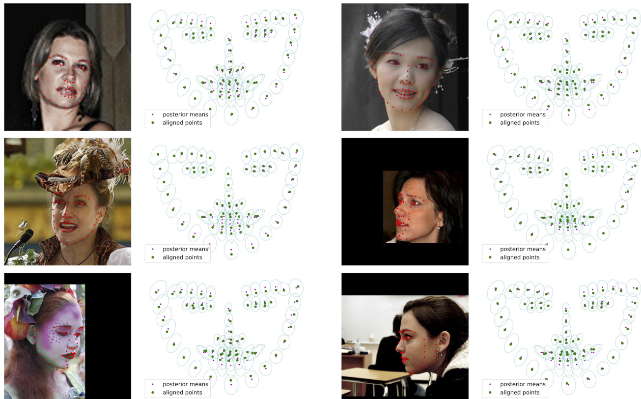
Fig. 14: Some examples of the best scores obtained with GStudent-EM and the ground-truth landmarks.
