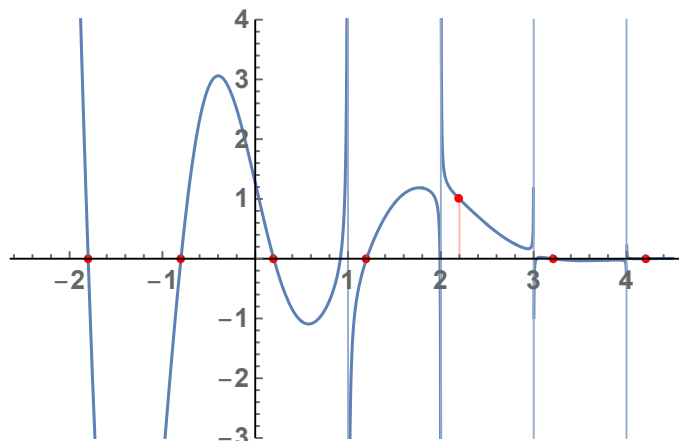
Figure 1. A plot of J^{(C)}(\alpha, \beta) with \beta = 2.2 as a function of (real) \alpha . We observe the kinematic poles at positive integer \alpha . The red dots help to show that J^{(C)}(\beta + n, \beta) = \delta_{n,0} .
