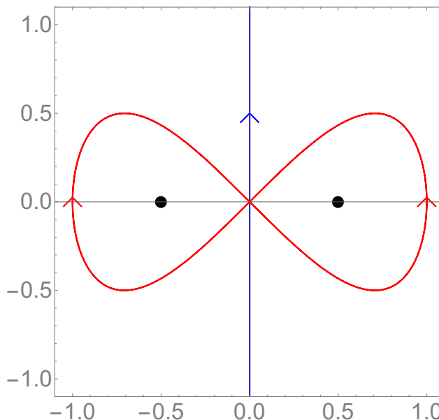
Figure 7. Plotted are the contours for the integral eq. (A.14). The blue contour gives \log(1-z) whereas the figure-of-eight red one gives 2(1-\log(z)) . The double poles at \alpha = \pm 1/2 are marked by black dots.
