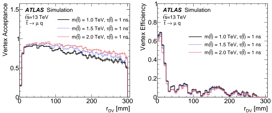
Figure 3: Vertex selection acceptance (left) and efficiency (right) are shown for the \tilde{t} R -hadron benchmark model as a function of the true transverse decay position r_{DV} .
