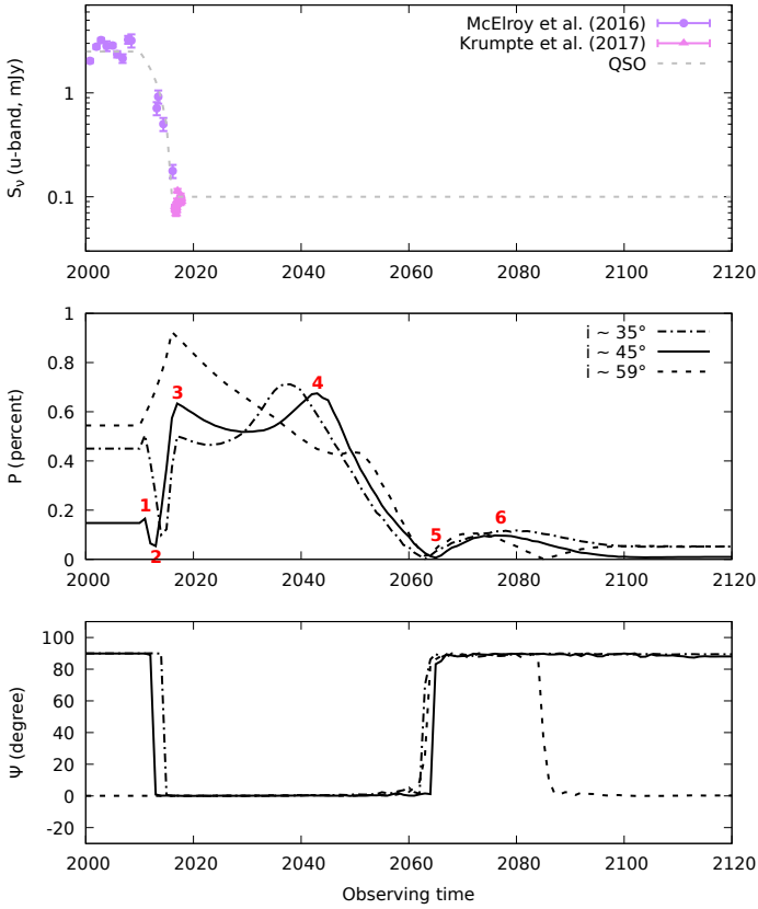
Fig. 6. Top panel: time series of archival u -band flux density S_\nu for the AGN in Mrk 1018 (McElroy et al. 2016; Krumpe et al. 2017). The host galaxy contribution has been carefully removed by the authors. We plot in gray the flux function we used in our simulation to mimic the dimming of the AGN (host contribution removed). Middle and bottom panels: model predictions for the polarization degree and polarization angle for different nuclear inclinations. See text for an explanation of the red numbers.
