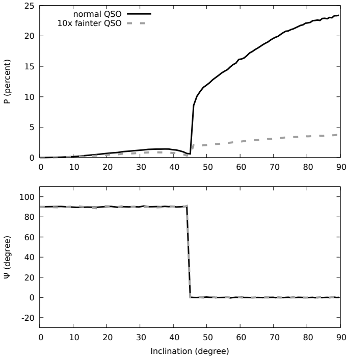
Fig. 2. Polarization degree ( top ) and polarization position angle ( bottom ) from our AGN model. The black line corresponds to a bright quasar. In this case, the host galaxy contributes \sim 5\% of the total light along type 1 inclinations ( i \leq 45^\circ ). The long-dashed gray line corresponds to the exact same quasar, but ten times fainter. The small fluctuations in P are due to statistical noise.
