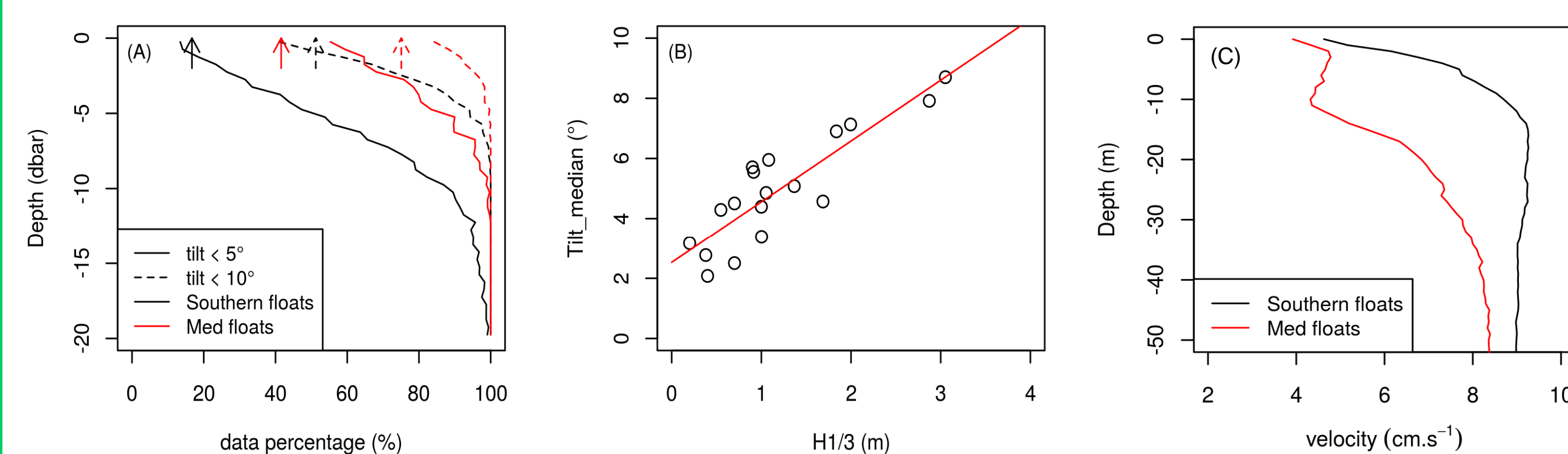
Fig. 2 (a, b, c) : navigation performances
