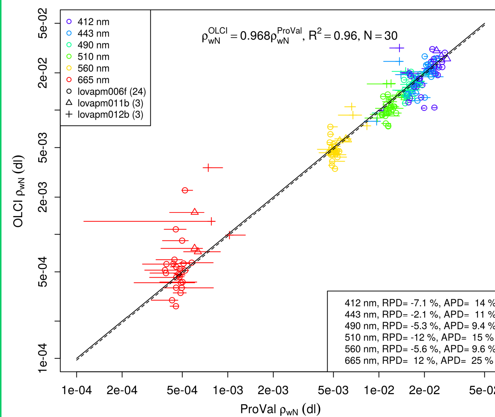
Fig 3 : normalized reflectance \rho_{wN} from OLCI and ProVals for both Mediterranean ( lovapm006f ) and Southern Ocean floats ( lovapm011b and lovapm012b ).
