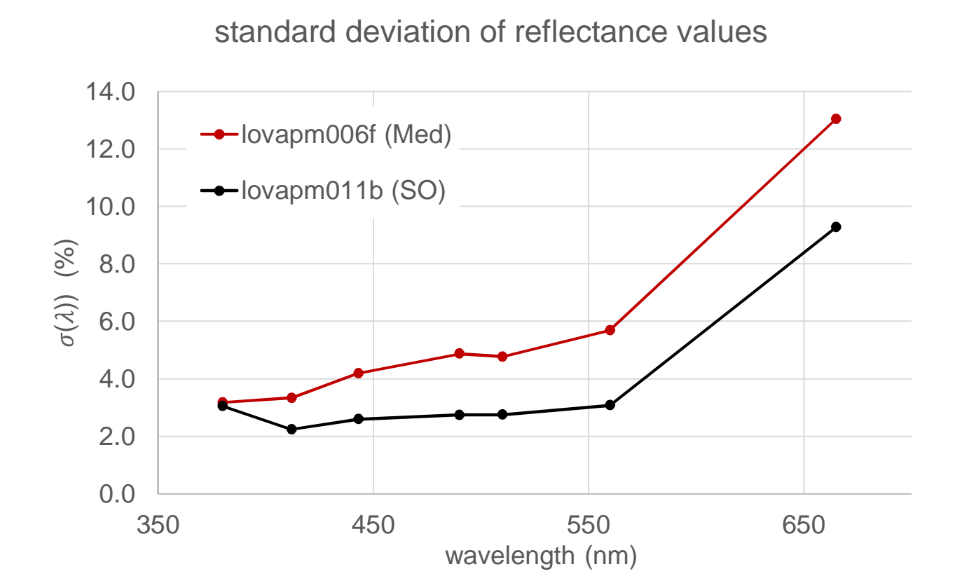
Fig 5 : standard deviation of Rrs normalized values for all profiles of floats lovapm006f and lovapm011b .
