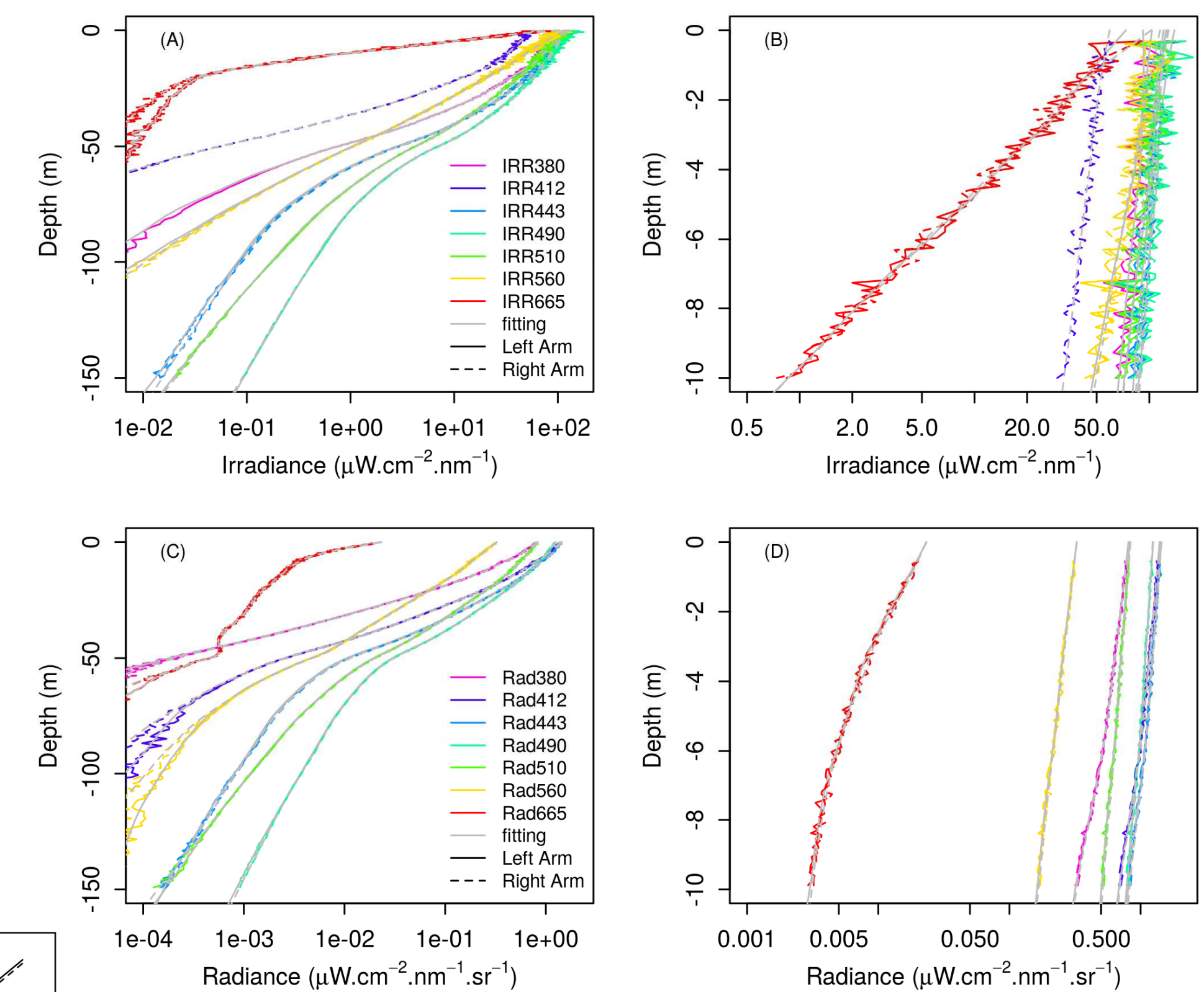
Fig 4 : Example of data, float lovapm006f (profile 57, 2017-08-02)
