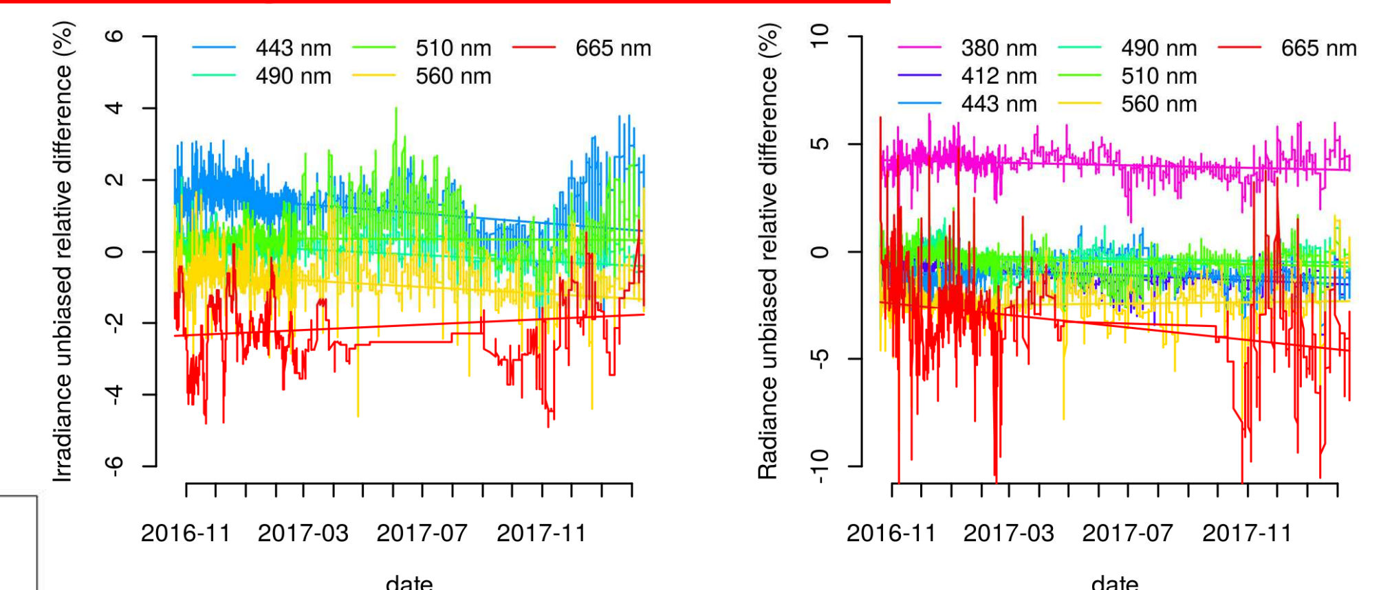
Fig. 6 : sensor relative difference between arms ( E_d and L_u , lovapm011b )
