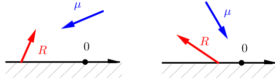
FIGURE 1. Two examples of parameters satisfying the inequality in (1) and (2). \mu is the drift and R is the reflection vector
