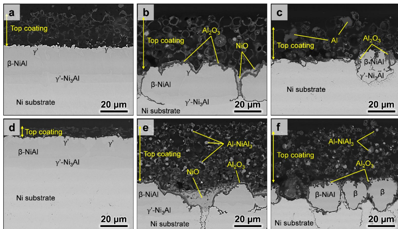
Figure 9 – BSE cross-section images of the thermal barrier systems elaborated from (a, b, c) Al_HS and (d, e, f) Al_DS microparticles on pure nickel after the complete heat treatment (700°C-2 h + 1100°C-2 h) in (a, d) Ar, (b, e) synthetic air and (c, f) Ar-10% H_2O .
