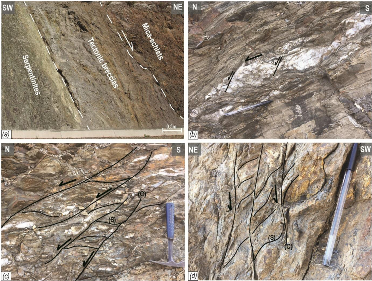
Fig. 4. Field photographs of the Aaraben area deformation. (a) the damaged zone of the Aaraben fault marked by a cataclasite corridor (N35°16'05", W04°50'23"). (b) Asymmetric boudinage of quartz-veinlet in a shear zone affecting the Filali mica-schists (N35°16'56", W04°51'25"). (c) extensional shear band in the mica-schists (N35°16'57", W04°51'25"). (d) S/C fabric in the serpentinized peridotite at the contact with the Filali unit (N35°16'52", W04°51'34").
