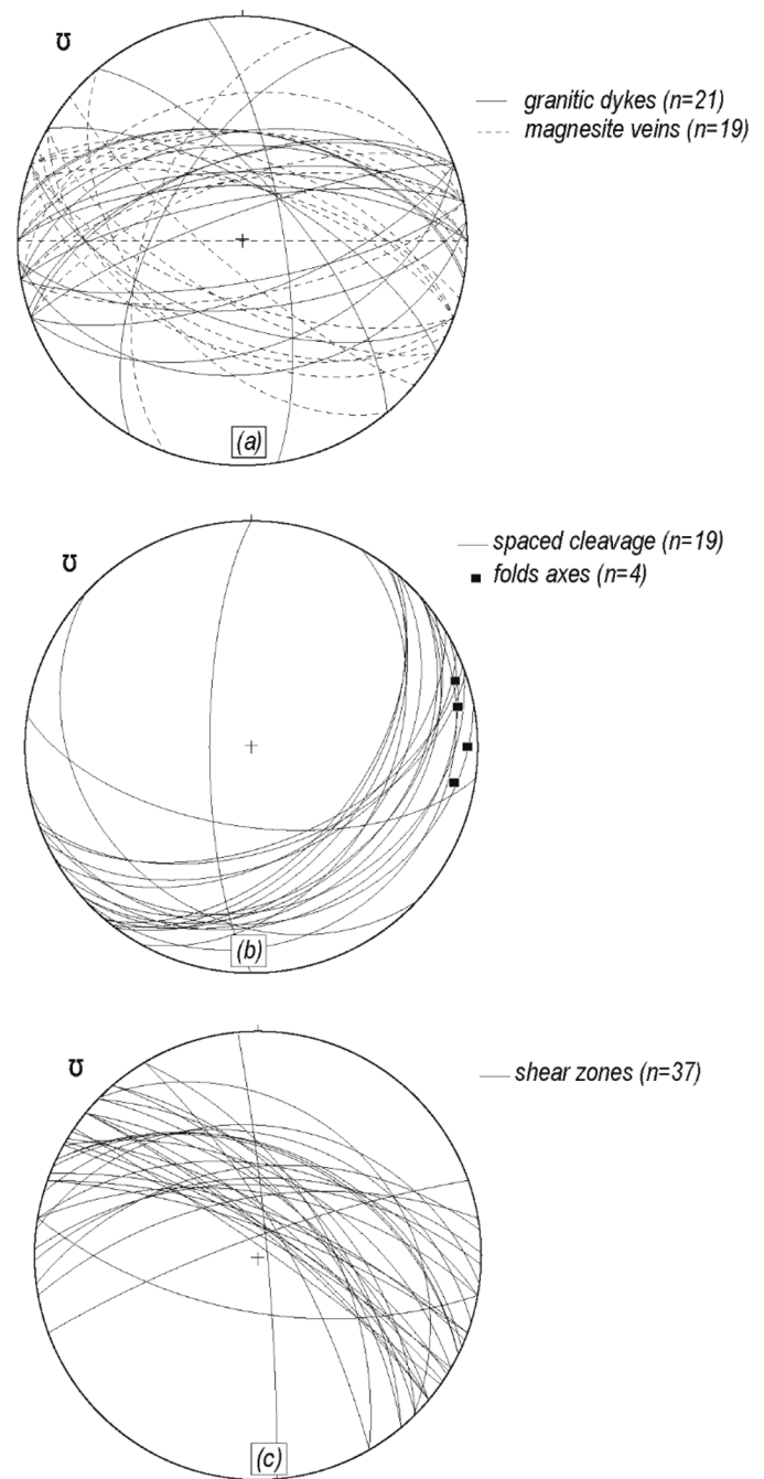
Fig. 5. Statistical distribution plot of structures in Beni Bousera massif. (a) granite dykes and magnesite veins. (b) spaced disjunctive cleavage and the folds axes. (c) shear zones in the NE of the Aaraben fault. Equal area projection, lower hemisphere.
