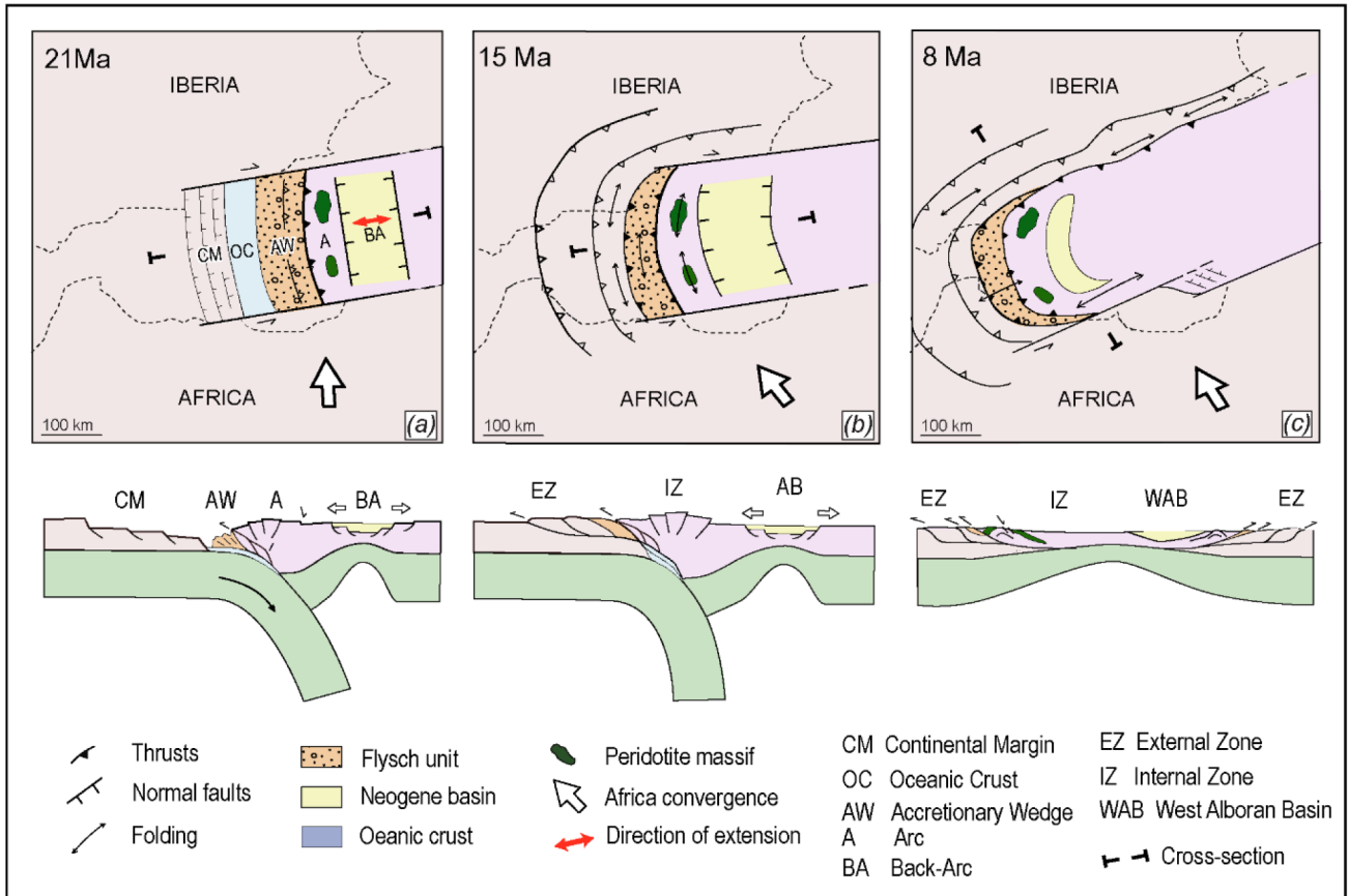
Fig. 10. Cartoons showing Miocene paleogeographic evolution of the Alboran Basin (map and cross-section) adapted from reconstructions by Do Couto et al. (2016), Crespo-Blanc et al. (2016) and Jolivet et al. (2019). The cross-sections (a) and (b) are E-W trending while the (c) cross-section is N-S trending.
