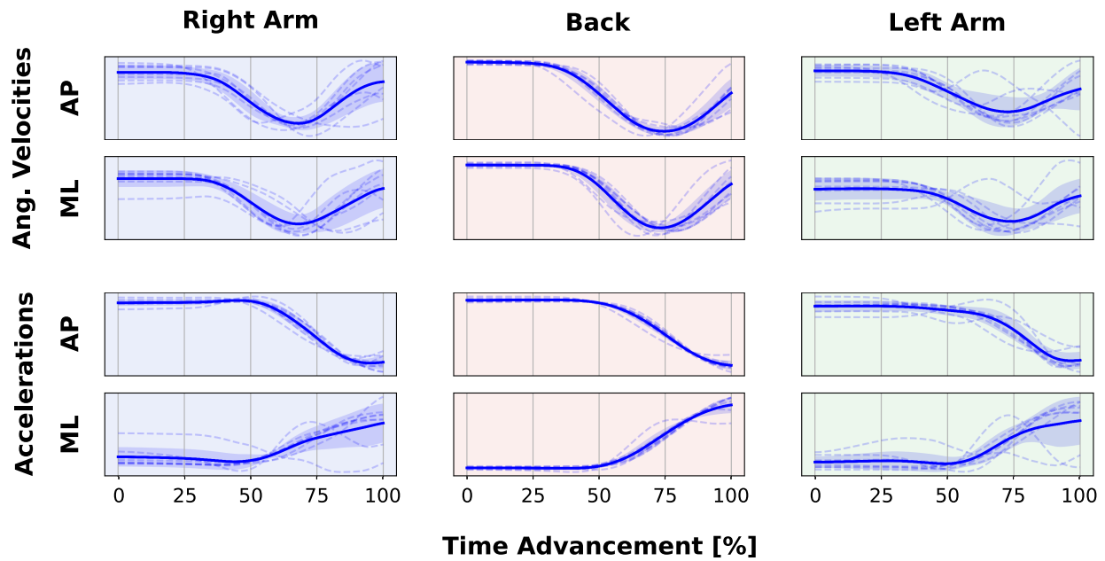
Fig. 4. Average accelerations and angular velocities recorded by all three IMUs during the CS condition trials in the ML and AP planes. The dashed lines represent the average signals for each subject, and the thick line corresponds to the overall average, with its corresponding standard deviation. Signals are represented from 0.5 s before the movement onset up to the first zero-crossing of the angular velocity around the vertical axis (not shown here).
