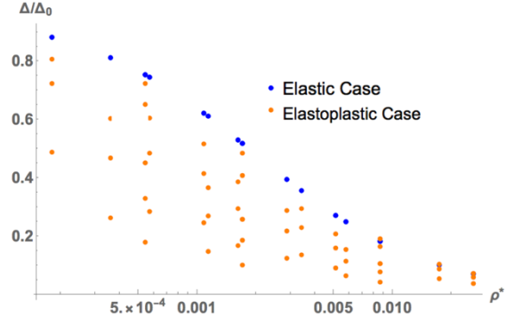
Figure 9. Deflection transmission ratio \Delta/\Delta_0 versus the relative stiffness \rho^* for elastic/elastoplastic behaviour of soil for various soil bearing capacities.
