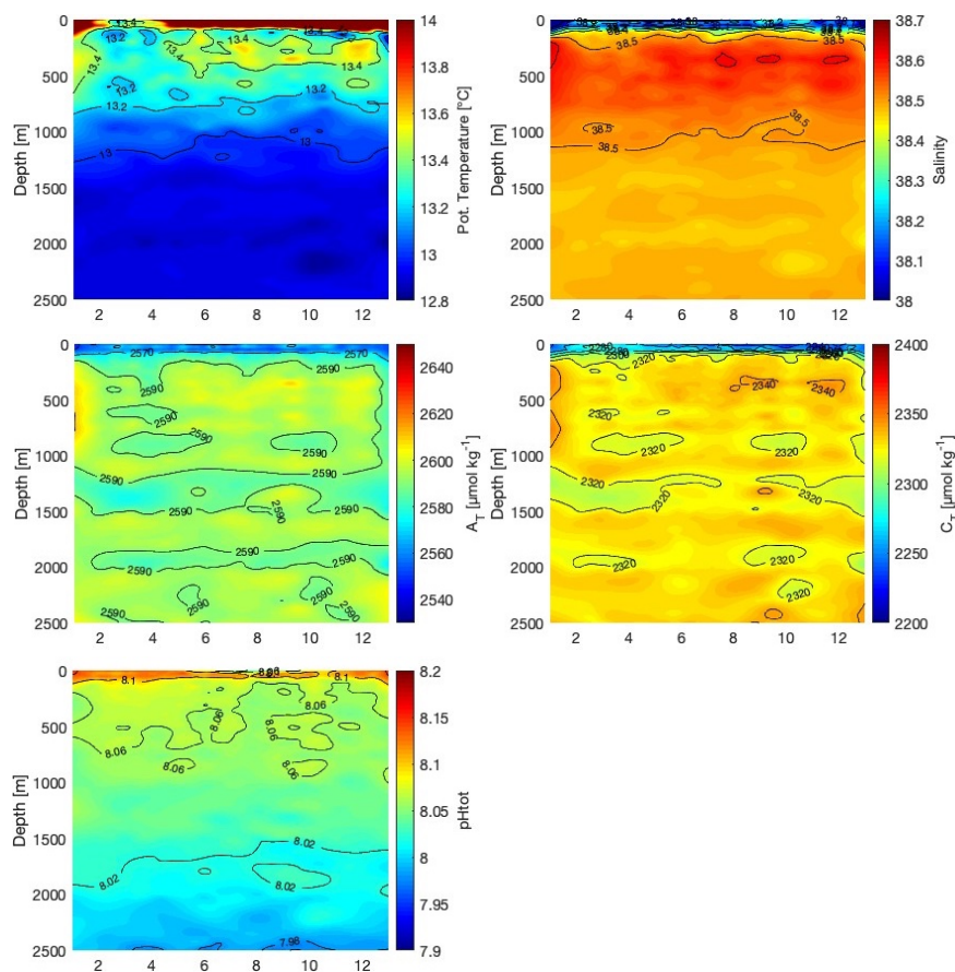
Figure 2. Water column monthly climatology of potential T , S and carbonate variables ( A_T , C_T and \text{pH} at total scale) in the Ligurian Sea derived from cruises conducted from 1998 to 2016 (all stations shown in figure 1). In the Ligurian Sea, the average C_T concentration ranges from 2200 in surface to 2350 \mu\text{mol kg}^{-1} in deep waters). Total alkalinity follows the same pattern with depth and ranges from 2500 to 2600 \mu\text{mol kg}^{-1} . \text{pH} (total scale) is higher in the upper 100 m (8.15) and decreases progressively with depth (< 8 in deep waters). Based on all dataset in 1998-2016 (about 1200 samples in deep waters) the mean C_T and A_T below 300 m are respectively 2328 \pm 9 and 2593 \pm 7 \mu\text{mol kg}^{-1} . In the next section we will also explore whether changes can be detected in deep layers.
