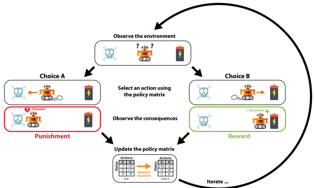
Fig 3. Illustration of a Partially Observable Markov Decision Process (POMDP). Given the current state of the environment, the agent takes an action by following the policy matrix, which is iteratively updated by the Bellman equation. The agent receives a triggered reward and observes the next state. The process goes on until interrupted or a goal state is reached.
