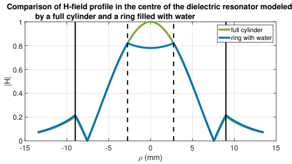
Fig. 9. H-field (absolute value of the total field) decrease in water (semi-analytical method). Full (respectively dashed) lines indicate the outer (resp. inner) boundaries of the ceramic probe. The penalty factor \tau defined in III is here estimated by the value of the blue curve in \rho = 0 .
