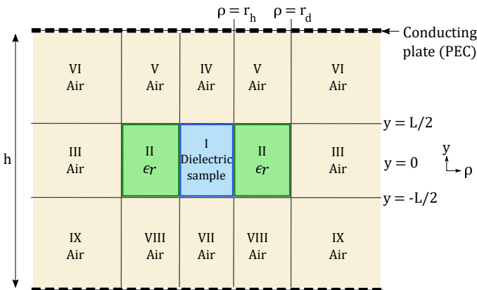
Fig. 5. Part by part space subdivision for field estimation.
