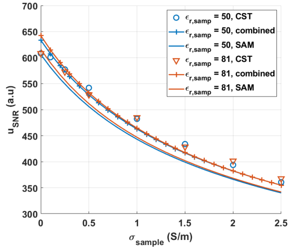
Fig. 12. Comparison, in terms of SNR factor, of semi-analytical model (SAM) with numerical simulations results (Frequency domain solver of CST Microwave Studio) and Eq. (28) applied to the E-field distribution from the software Eigenmode solver (combined).
