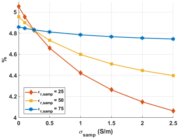
Fig. 11. Comparison of semi-analytical model and numerical simulations results in terms of normalized power losses term \tau^2 P_{loss,norm}^{sample} + P_{loss,norm}^{ring} , as a function of the sample conductivity.
