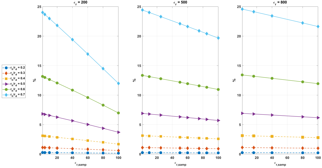
Fig. 4. Quantification of the TE_{01\delta} mode frequency shift between the disk resonator and the dielectric probe (for both, numerical simulations results with CST Eigenmode Solver). The probe ring has its relative permittivity equal to 200 (left), 500 (center) and 800 (right). The frequency variation is plotted as a function of the sample permittivity and for several discrete values of the radii ratio. Curves in dashed lines correspond to systematic frequency shift inferior to 5%.
