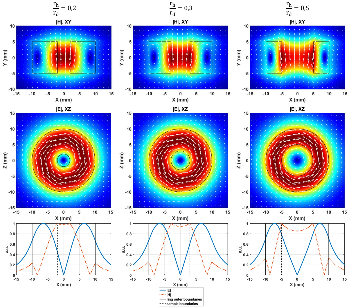
Fig. 7. Normalized field maps for a dielectric ring (permittivity 500, height 10 mm, outer diameter 20 mm) filled with a sample of permittivity 50 for different inner to outer radii ratios. Top line: modulus of the total magnetic field. Middle line: modulus of the total electric field. Bottom line: field lines of the total electric (blue solid line) and magnetic (orange dotted line) fields in the center of the resonator ( y = 0 ). The maps and field lines are normalized to the maximum value of the field modulus. Linear color scale from 0 to 1.
