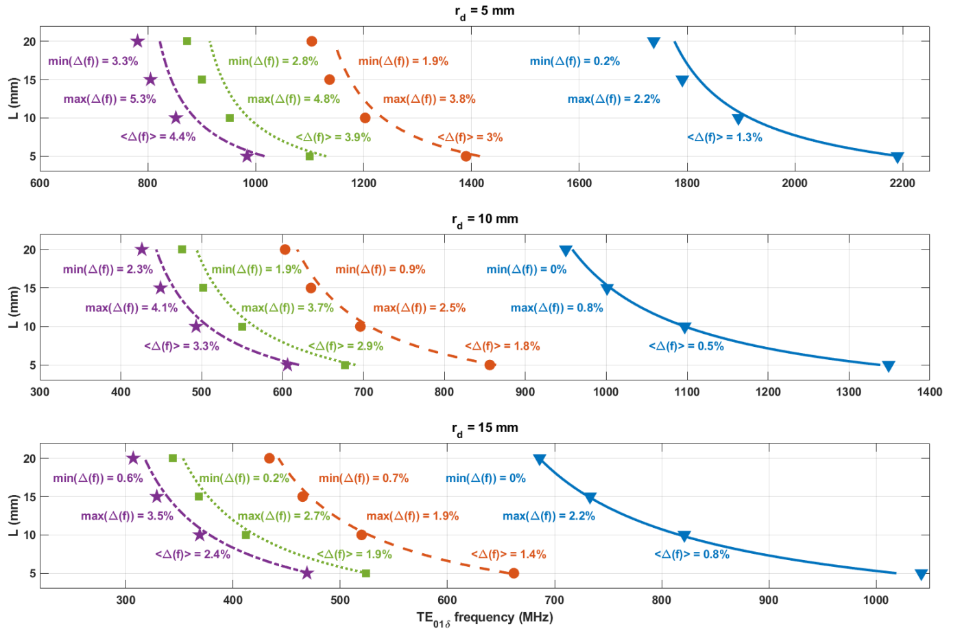
Fig. 3. Comparison between numerical simulations and semi-analytical method (Eq. (4)) of TE_{01\delta} eigenmode frequency estimation as a function of the disk height ( L ), radius ( r_d ) and permittivity (blue: 200, orange: 500, green: 800, purple: 1000). Lines represent the results from the semi-analytical method proposed in this paper ( f_{res} , Eq. (4)), and markers represent CST results. For each curve, the maximum, minimum and averaged value of the relative error \Delta(f) are indicated.
