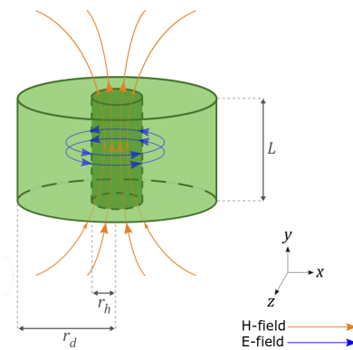
Fig. 2. TE_{01\delta} mode of a ring resonator (schematic field lines), notations and coordinates system
