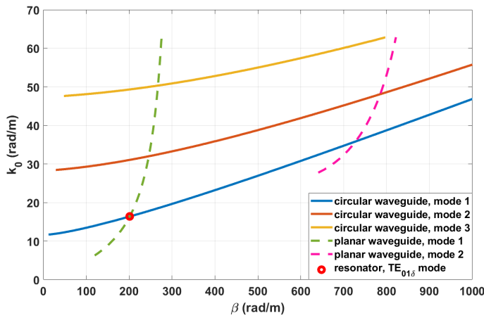
Fig. 6. Dispersion curves of the infinite dielectric circular (solid lines) and planar (dashed lines) waveguides corresponding to the cylindrical resonator from Reference [23] (with \epsilon_{r,\text{samp}} = 50 ). Only the three (respectively two) first modes of the circular (resp. planar) waveguide can be seen in the considered ranges of frequencies and \beta values. The first TE mode of this ring resonator is shown with a red circle at the intersection point of the first waveguides modes.
