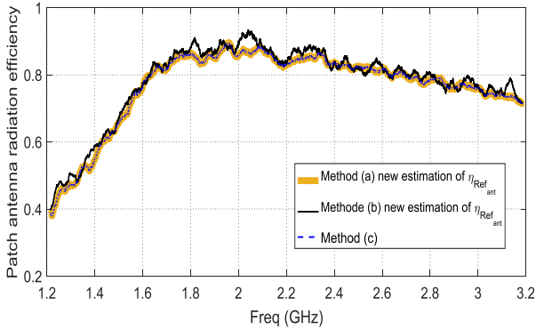
Fig. 7. Patch antenna radiation efficiency with the new estimation of \text{Ref}_{\text{ant}} radiation efficiency.
