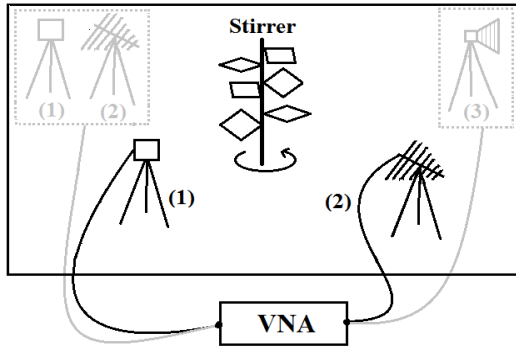
Fig. 3. Measurement Setup.
