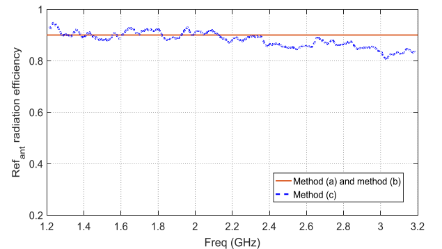
Fig. 6. Log periodic ( Ref_{ant} ) radiation efficiency. Its value is supposed fixed and equal to 90% for methods (a) and (b) whereas it is measured using method (c).
