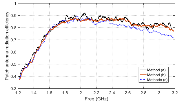
Fig. 5. Patch antenna radiation efficiency using the three methods versus frequency.
