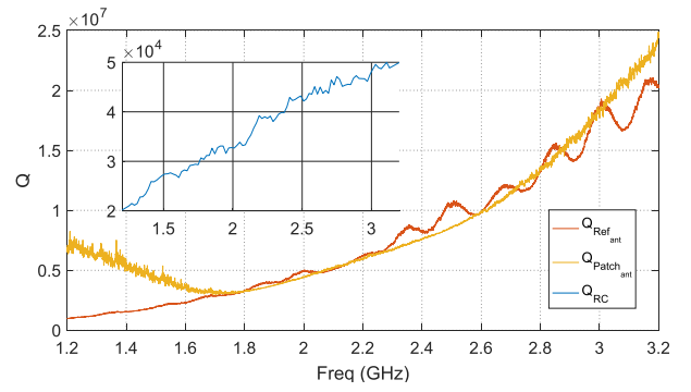
Fig. 4. RC and antennas quality factors.
