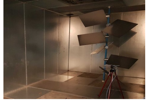
Fig. 1. RC of IETR laboratory.
