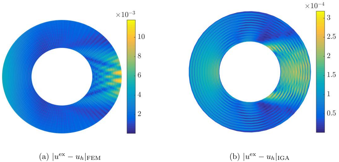
Figure 6: Absolute error |u^{\text{ex}} - u_h| for k = 40 , p = 3 , n_\lambda = 10 . The numerical error with IGA is considerably lower for the identical basis order, number of degrees of freedom and the integration points. The contribution of the domain truncation error was eliminated by considering BGT-2 type ABC and modified exact solution.
