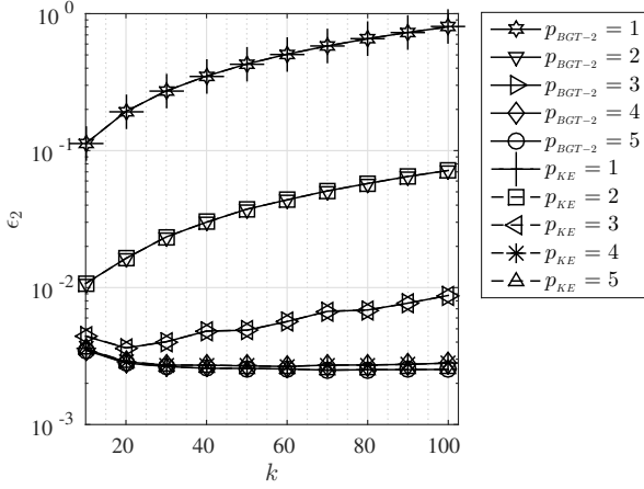
(a) BGT-2 is equivalent to KFE for NT = 1
