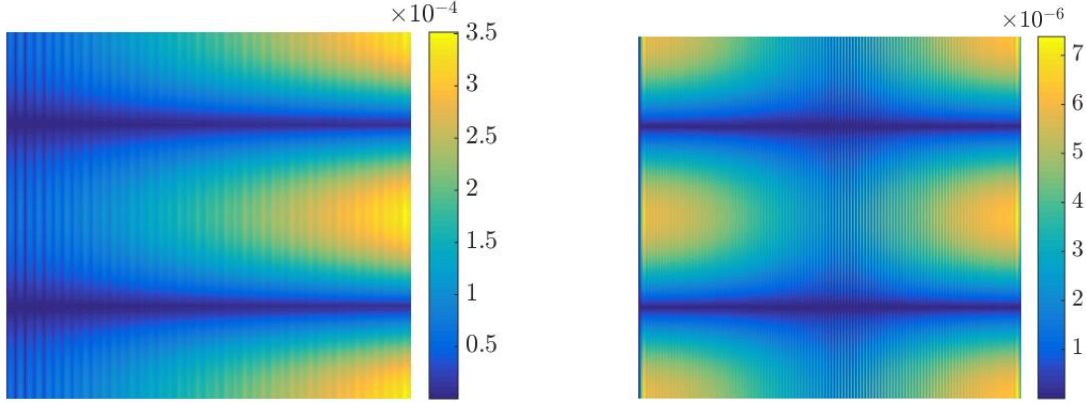
(a) |u^{\text{ex}} - u_h|_{\text{FEM}}
