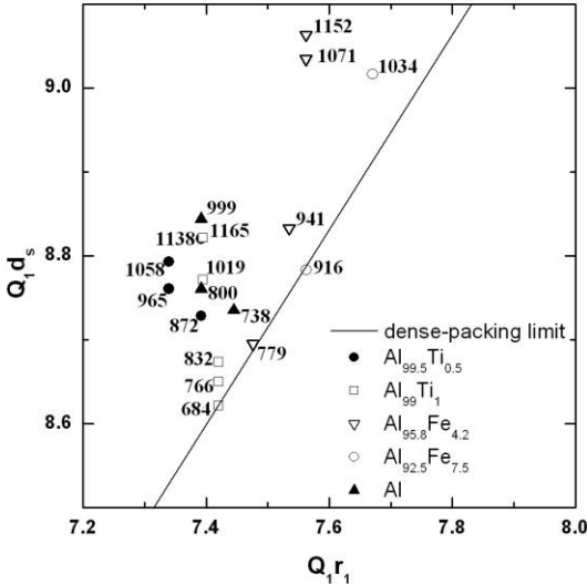
Figure 9. Scattering vectors of the first peaks in the structure factors S(Q) of liquid alloys, scaled by the nearest-neighbor distance r_1 and the mean interatomic spacing d_s . The values near the data points indicate the temperature in °C.
