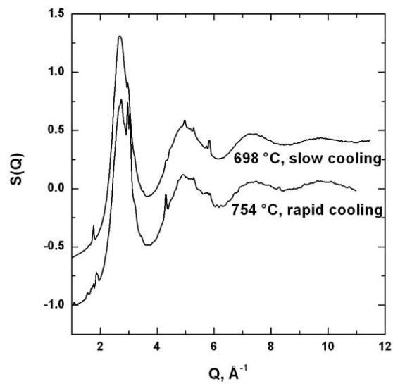
Figure 4. The dependence of the crystallization of intermetallic \text{Al}_{13}\text{Fe}_4 from the cooling rate in \text{Al}_{92.5}\text{Fe}_{7.5} alloy.
