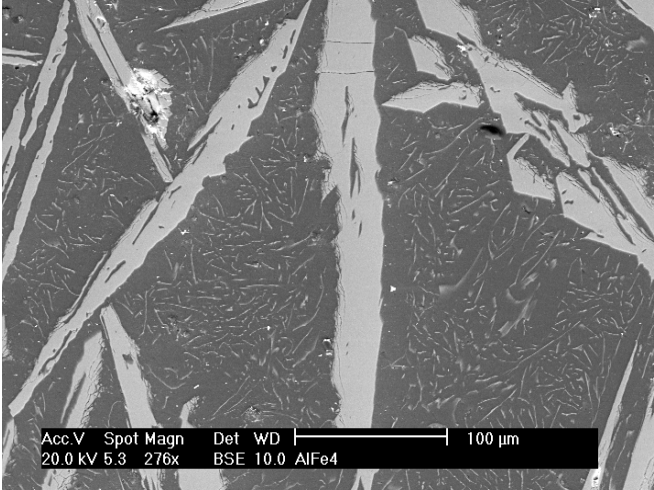
Figure 7. SEM image of the microstructure in Al 95.8 Fe 4.2 alloy.
