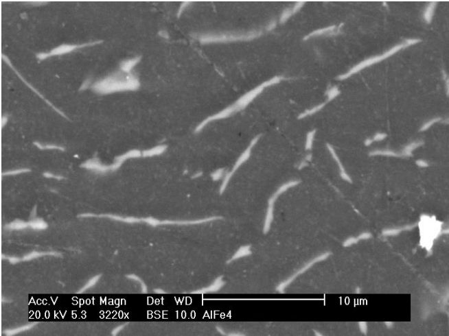
Figure 8. SEM image of the microstructure in Al 95.8 Fe 4.2 alloy with higher magnification.
