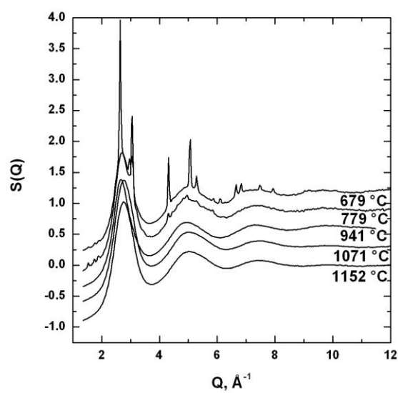
Figure 2. Average x-ray structure factor S(Q) for liquid \text{Al}_{95.8}\text{Fe}_{4.2} at different temperatures. Spectra are shifted vertically for clarity. At 779 °C and 679 °C the sample was partly solid.
