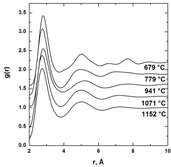
Figure 6. Average pair correlation function g(r) for liquid \text{Al}_{95.8}\text{Fe}_{4.2} at different temperatures. The g(r) curves are shifted vertically for clarity. At 779 °C and 679 °C, the sample was partly solid.
