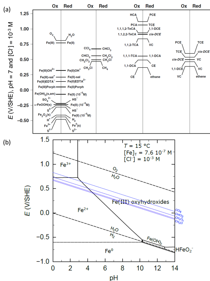
Figure 6.1. (a) Oxidation-reduction potential (ORP) of iron and sulfur species and chlorinated methanes, ethanes and ethylenes at pH = 7 and [Cl^-] = 10^{-3} M (from Cwiertny and Scherer (2010), adapted from Schwarzenbach et al. (2003)). (b) Simplified Pourbaix diagram for Fe/H 2 O system under reference conditions (adapted from Matheson and Tratnyek 1994; T = 15 °C, [Cl^-] = 10^{-3} M, [Fe]_T = 7.6 \cdot 10^{-7} M).
