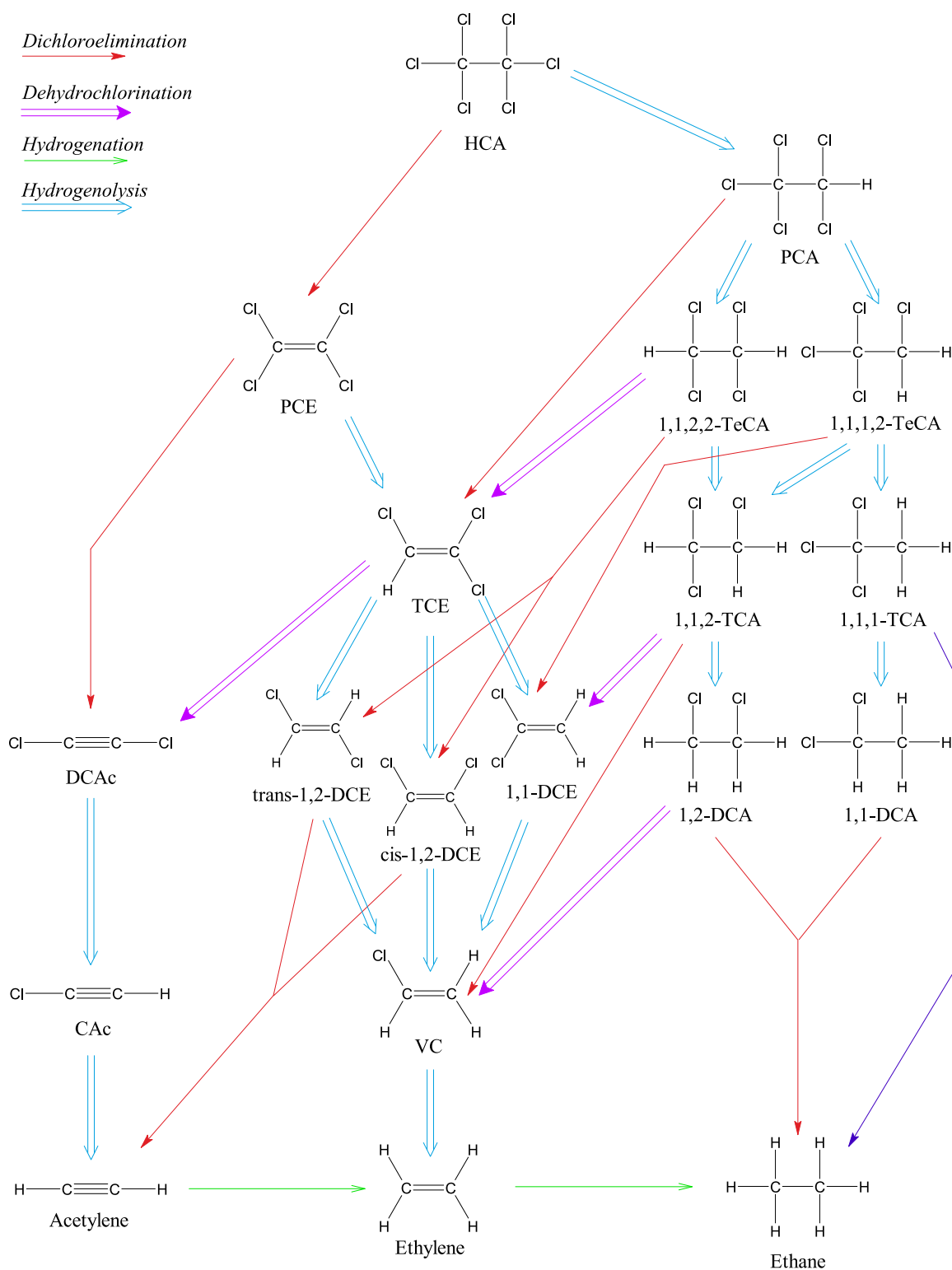
Figure 6.3. Reductive dechlorination pathways of HCA by ZVI.
