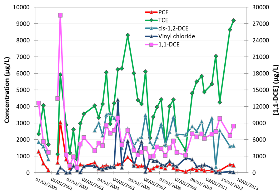
Figure 6.10. COCs content evolution at piezometer F5 inside the polluted zone between 2000 and 2013.
