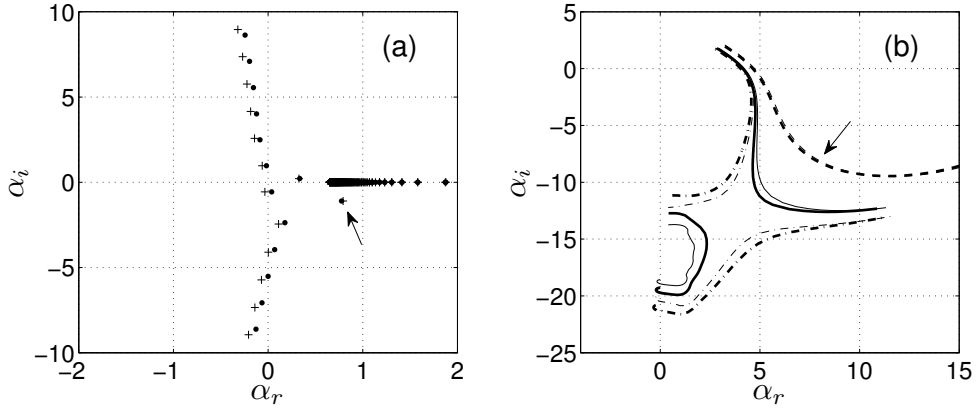
Figure 8: (a) Spectra obtained at \omega = \omega_a = 0.196 : + compressible case Eq. (30) ; • incompressible case Eq. (31). (b) Trajectories of the unstable mode along several L_\omega contours: -.- \omega_{L,i} = 0.10 compressible; — \omega_{L,i} = 0.11 compressible; - - - \omega_{L,i} = 0.12 compressible; -.- \omega_{L,i} = 0.10 incompressible; — \omega_{L,i} = 0.11 incompressible; - - - \omega_{L,i} = 0.12 incompressible.
