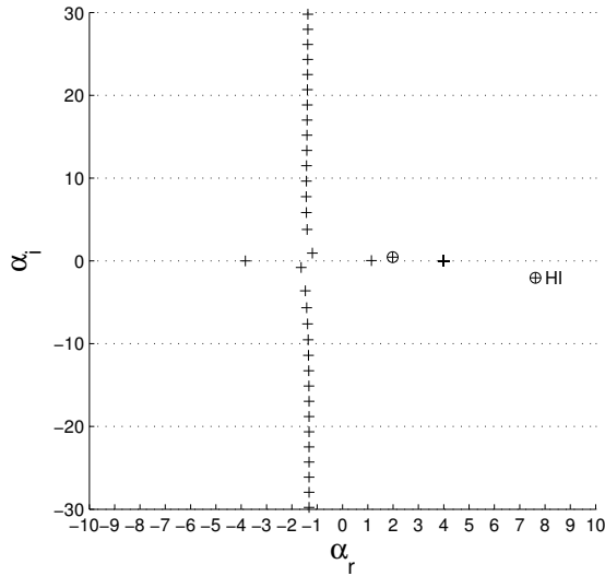
Figure 5: Spectrum for: M_0=0.5 , \omega=2 , Y=2.5-2.5i . The plug flow and Myers boundary condition are used together. Symbols: + present numerical method with N=100 Chebyshev modes; o asymptotic approximation for surface waves as given by roots of Eq. (36). The numerical value for the Hydrodynamic Instability (HI) mode is given in table 1.
