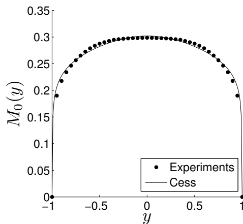
Figure 2: Experimentally measured mean velocity profile; and analytical approximation obtained by integration of Eq. (3) using Cess' expression for the total viscosity, Eq. (4).
