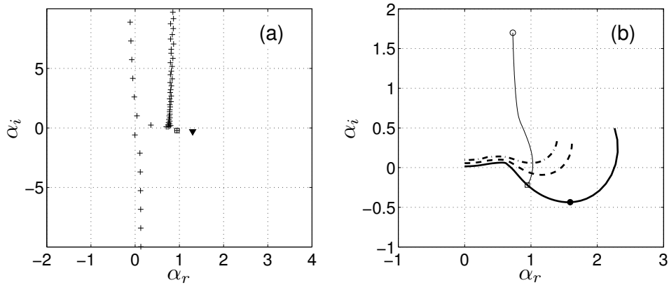
Figure 9: (a) Spectrum obtained at \omega=\omega_a=0.196 by solving Eq. (32). The symbol \square indicates the convectively unstable mode. The symbol \blacktriangledown indicates the experimental unstable mode. (b) Trajectories of the unstable mode along several L_\omega contours: — \omega_{L,i}=0 ( \omega real); - - - \omega_{L,i}=0.0009 ; - · - \omega_{L,i}=0.0018 . The line — represents the trajectory of the unstable mode when the imaginary part of \omega is increased from 0 ( \square symbol) to 0.41i ( \circ symbol), the real part being fixed at \omega_r = \omega_a . The symbol \bullet is for the mode having maximal growth rate for \omega real.
