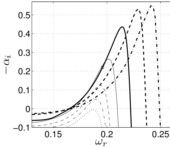
Figure 12: Spatial growth rate for the spatially unstable branch as a function of \omega_r for several values of the section-averaged Mach number: \dots M_{0,\text{avg}}=0.16 ; -\cdot-\cdot- M_{0,\text{avg}}=0.165 ; - - M_{0,\text{avg}}=0.18 ; — M_{0,\text{avg}}=0.21 ; — M_{0,\text{avg}}=0.27 ; -\cdot-\cdot- M_{0,\text{avg}}=0.36 ; -\cdot-\cdot- M_{0,\text{avg}}=0.45 . The symbol \square indicates the convectively unstable mode at the baseline value M_{0,\text{avg}}=0.27 and \omega=\omega_a=0.196 .
