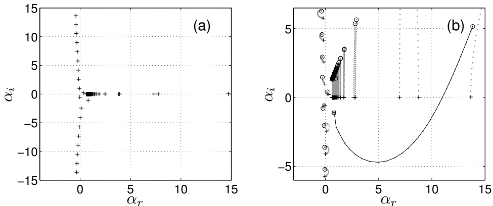
Figure 6: (a) Spectrum calculated by solving (30) for \omega = \omega_a = 0.196 . (b) Trajectories of the modes when the imaginary part of \omega is increased from 0 to 0.41i , the real part been kept constant at \omega_r = \omega_a . The symbols + indicate the starting points for \omega_i = 0 (the same as in (a)); the symbols o indicates the points for \omega_i = 0.41 . The gray dots are for the trajectory in between. The symbol \square indicates the potentially unstable mode. The line — obtained with the shooting method is a further verification of the trajectory of the potentially unstable mode.
