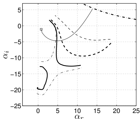
Figure 7: Trajectories of one selected branch \alpha(\omega) for \omega belonging to L_\omega contours with: - - \omega_{L,i}=0.10 ; — \omega_{L,i}=0.11 ; - - - \omega_{L,i}=0.12 ; - . - \omega_{L,i}=0.18 ; - - - \omega_{L,i}=0.41 . The curve — is the trajectory of the branch for \omega_r=\omega_a and \omega_i increasing from 0 to positive values (this is the same as in Fig. 6(b)).
