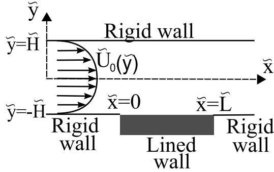
Figure 1: Studied configuration. The notation \tilde{\cdot} is for physical quantities
