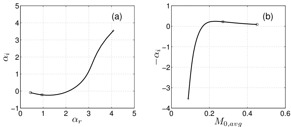
Figure 11: (a) Trajectory of the unstable mode and (b) Growth rate as a function of the section-averaged Mach number, obtained at \omega = \omega_a = 0.196 when varying the section-averaged Mach number from M_{0,avg} \sim 0.09 (+ symbol) to \sim 0.45 (o symbol). The symbol \square indicates the convectively unstable mode at the baseline value M_{0,avg} = 0.27 .
