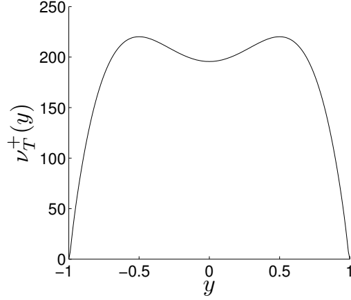
Figure 3: Total viscosity, given by Eq. (4) for \text{Re}_\tau=2760 .
