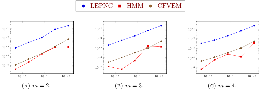
FIGURE 7. Locally refined Cartesian meshes: fraction of negative mass N_{\text{Mass}} versus mesh size.
