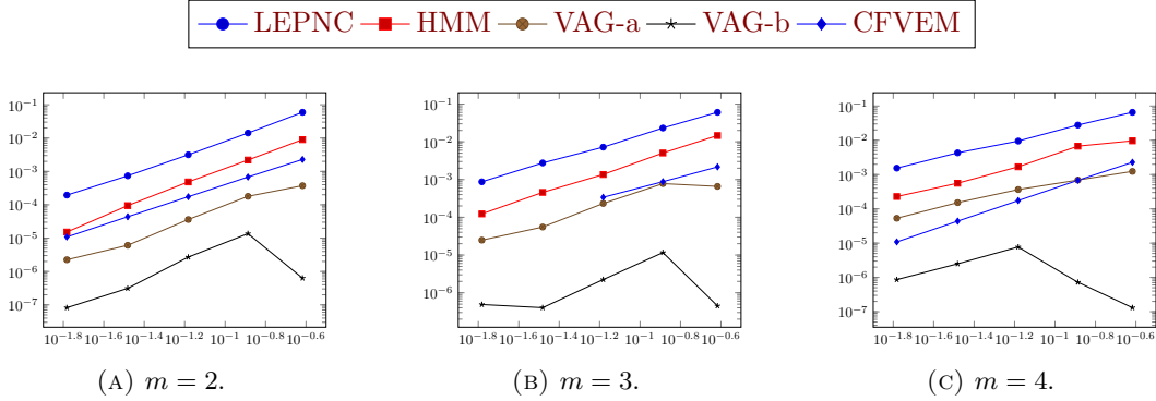
FIGURE 6. Hexagonal meshes: fraction of negative mass N_{\text{Mass}} versus mesh size.
