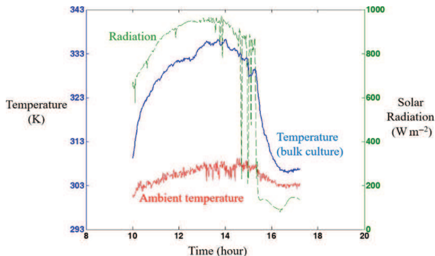
FIG. 26.8 Typical thermal behavior of a flat panel system during a sunny day in France (Perpignan, July 2010). To emphasize the overheating, the system was operated without thermal regulation (water solution and black dye).
