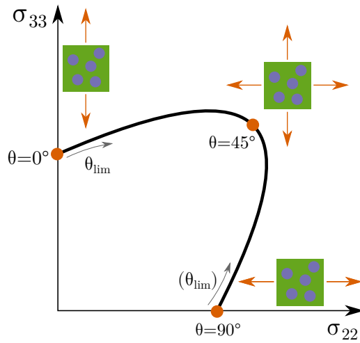
Figure 12: Illustration of a biaxial yield envelope. The angle \theta defines the ratio between the two stress components. When training surrogates, \theta_{lim} is used to define the bounds of the training space.
