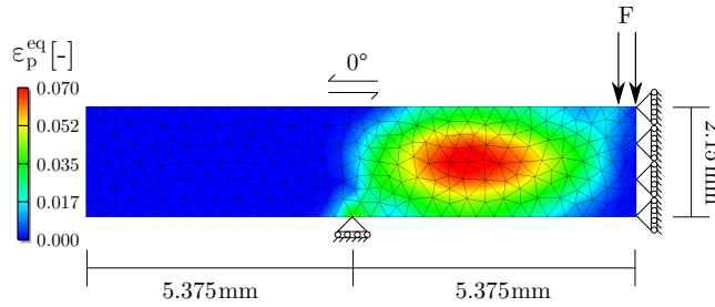
Figure 27: Short-beam FE 2 example. Loads and boundary conditions are shown as well as the plastic strain field at the final time step.
