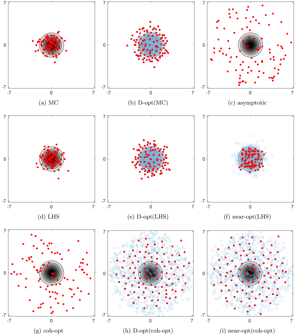
Figure 9: Visualization of the experimental design constructed for standard Gaussian input in d = 2 dimensions for degree p = 12 . The gray surface plot illustrates the Gaussian pdf. Red filled points denote the chosen experimental design, while blue circles denote the candidate set. Size of the ED: N = 100 , size of the candidate set: M = 1000 . The support of the asymptotic and the coherence-optimal distribution is the ball of radius r = \sqrt{2}\sqrt{2p+2} \approx 7.2 . Note that engineering models may be less accurate in regions where the input distribution has negligible mass.
