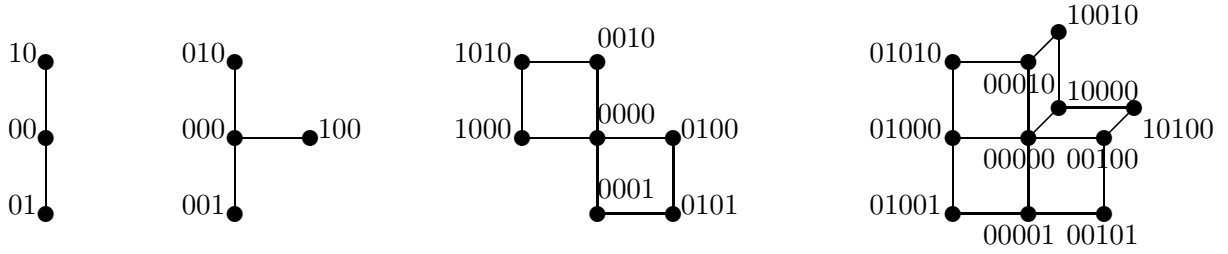
Figure 1: \Gamma_2 = \Lambda_2 , \Lambda_3 , \Lambda_4 and \Lambda_5
