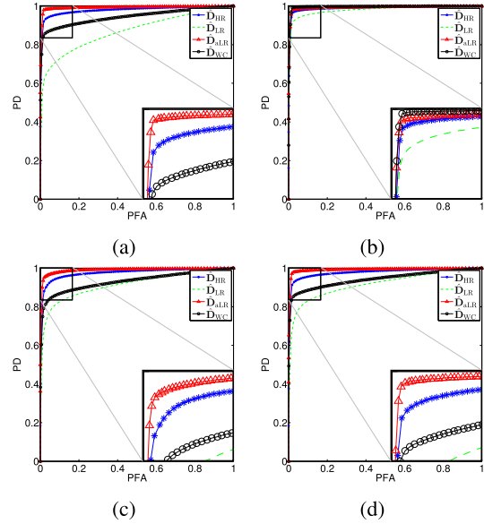
Fig. 5. Scenario 1 (SNR = 30 dB). ROC curves computed from (a) CVA, (b) sCVA(7), (c) MAD, and (d) IR-MAD.
