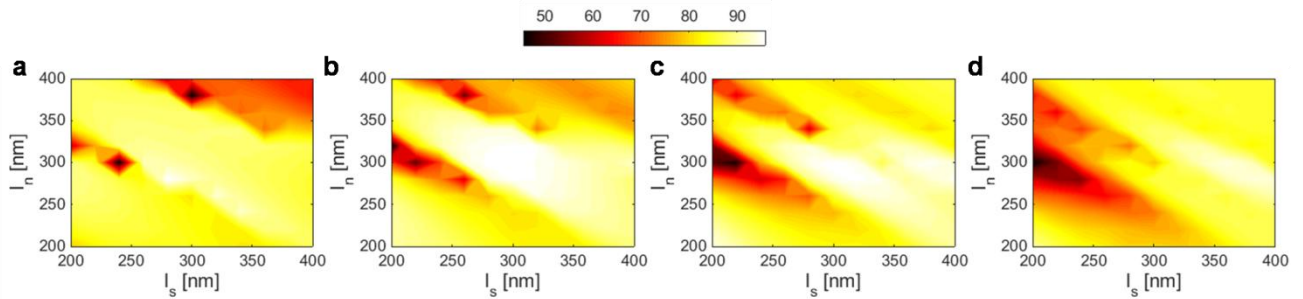
Figure 3. 2D mapping of the grating directionality versus lengths of the shallow-etch trenches and unetched teeth for various lengths of deep-etch trenches: (a) l_d = 50 nm; (b) l_d = 100 nm; (c) l_d = 150 nm; and (d) l_d = 200 nm.
