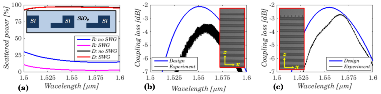
Figure 1. (a) Diffracted power from an L -shaped grating coupler as a function of wavelength. Inset: Vertical schematic of the L -shaped grating coupler. Calculated and measured coupling loss as a function of wavelength of the L -shaped grating couplers (b) without and (c) with sub-wavelength-engineered metamaterial transition. Insets of (b) and (c): Scanning electron microscopy images.
