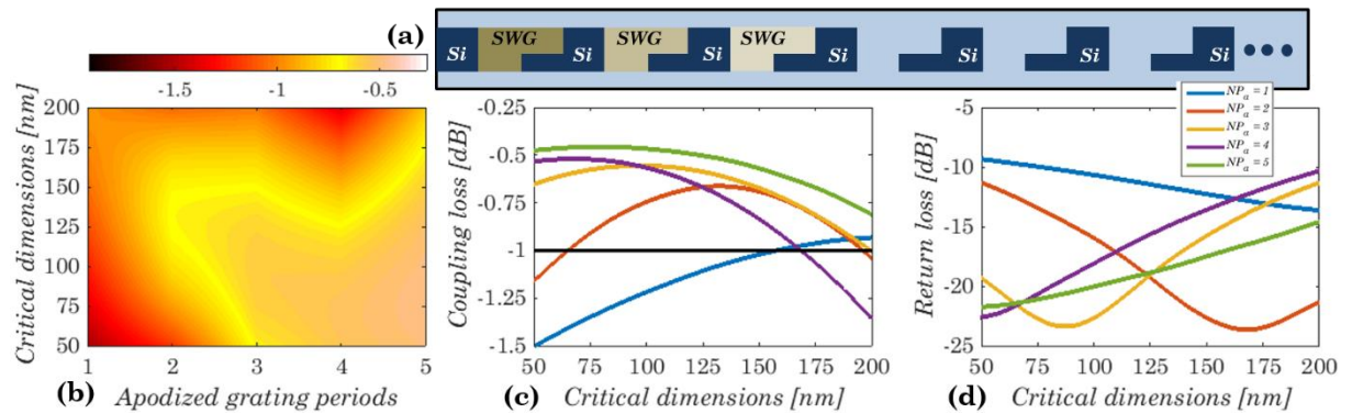
Figure 2. (a) Vertical schematics of an apodized L -shaped grating coupler with sub-wavelength-engineered trenches. (b) Colour map showing coupling loss of the L -shaped grating coupler as a function of the number of apodized periods and critical dimensions. (c) Coupling loss and (d) reflectivity of the L -shaped grating coupler as a function of critical dimensions for different numbers of apodized periods.
