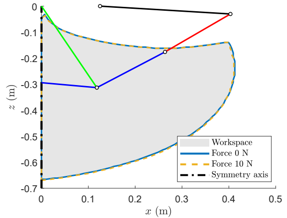
FIGURE 11: Contour of the Cartesian workspace corresponding to the projection of a single subset of solutions to the IGSP. The workspace is plotted for two cases, when no force is applied on the end-effector and when a force of 10N is applied downwards.
