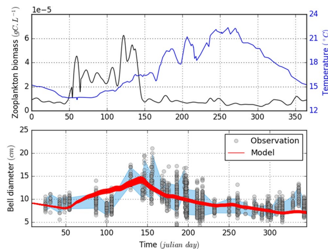
Figure 5. Comparison of jellyfish size variations between in situ observations and outputs of the model, based on fifty random simulations within the best parameters combinations defined by the SMCE. Subpanels show: (a) the annual sea surface temperature (blue) and annual zooplankton biomass (black) climatologies (from August 2011 to December 2015) that were used as model inputs; and (b) the jellyfish size variation obtained from in situ observations (dots) and model simulations (red lines). The blue color represents the tunnel of confidence for our SMCE decision.
