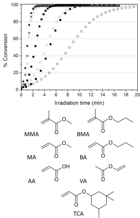
Figure 1. Conversion profiles of various miniemulsions photopolymerized by monomer self-initiation, the average droplet diameter determined by DLS is given in brackets: MMA ( \square , 77 nm), VA ( \blacksquare , 85 nm), BA ( \triangle , 100 nm), MA ( \star , 71 nm), TCA ( \ast , 210 nm), BMA ( \circ , 112 nm) and MMA/BA/AA: 49.5:49.5:1 wt % ( \bullet , 75 nm). SA or HD = 4 wt % / C_{\text{monomer}} , SDS = 3.5 wt % / C_{\text{monomer}} , C_{\text{monomer}} = 30 wt %. Optical path = 500 \mu\text{m} .
