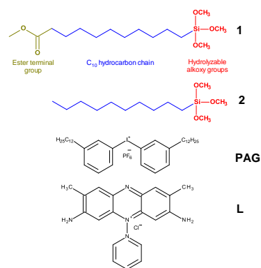
Scheme 1. Structures of monosilylated trimethoxysilane precursors ( 1 , 2 ), photoacid generator ( PAG ) and fluorescent amino-based ligand ( L )
