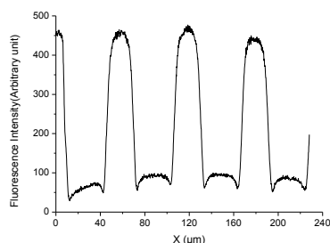
Figure 9. Image of the photopatterned 1-PHL film surface obtained with fluorescence microscopy (scale bar = 50 \mu\text{m} ).
