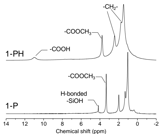
Figure 4. Solid state ^1H MAS NMR spectra of the hybrid films 1-P and 1-PH following ester hydrolysis
