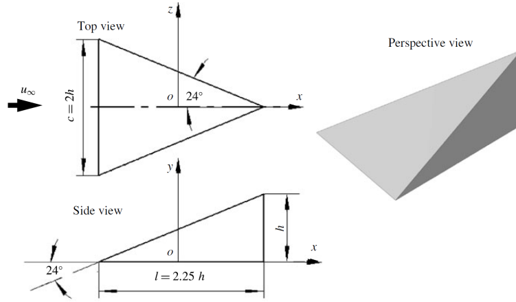
(a) Micro-ramp geometry and geometrical parameters (from [21])
