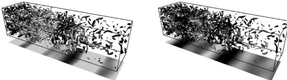
Fig. 13. Simultaneous injection of isotropic homogeneous turbulence and acoustic wave. Isosurface of Q criterion Q = 2.5(U/L)^2 colored by the axial velocity ( 95 \leq u(m/s) \leq 105 ) and fluctuating pressure in the range -1.2e - 2 \leq p/p_\infty - 1 \leq 1.2e - 2 in one plane. Left: NSCBC, right: NRI-NSCBC.
