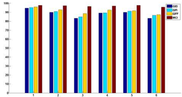
Fig. 5 Average classification rates for a fast gait from the CMU MoBo dataset yielded by the four gait representation methods: GEI, GFI, GFF, MCI (proposed method), distinguishing among the six camera viewpoints: 1 (v03), 2 (v05), 3 (v07), 4 (v13), 5 (v16) and 6 (v17), see Fig. 3
