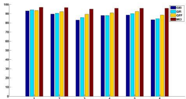
Fig. 7 Average classification rates for carrying ball gait from the CMU MoBo dataset yielded by the four gait representation methods: GEI, GFI, GFF, MCI (proposed method), distinguishing among the six camera viewpoints: 1 (v03), 2 (v05), 3 (v07), 4 (v13), 5 (v16) and 6 (v17), see Fig. 3
