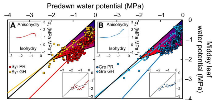
Fig. 1. \Psi_{\text{mdl}} depending on \Psi_{\text{pd}} in different V. vinifera varieties. Syrah (A) and Grenache (B) were measured in the field [domain “Pech Rouge” (PR); dark colors] and during a drydown experiment in greenhouse (GH; light colors). The slope \sigma of the linear regressions was not statistically different across varieties in the field ( P = 0.074 ) nor in the greenhouse ( P = 0.225 ). Top left insets represent the slope \sigma_x (sensitivity to declining water availability) depending on the range of \Psi_{\text{pd}} (from 0 to x ; x representing the lower limit of the range of \Psi_{\text{pd}} ) combining field and greenhouse data. Bottom right insets represent the correlation between \Psi_{\text{pd}} and minimum \Psi_{\text{mdl}} (that is, average value of three lowest \Psi_{\text{mdl}} per 0.1\text{-MPa} wide class of \Psi_{\text{pd}} ) combining field and greenhouse data. This linear regression is used to define the lower range of the hydroscape (colored by a blue-to-red gradient representing increasing water stress on the main figure).
