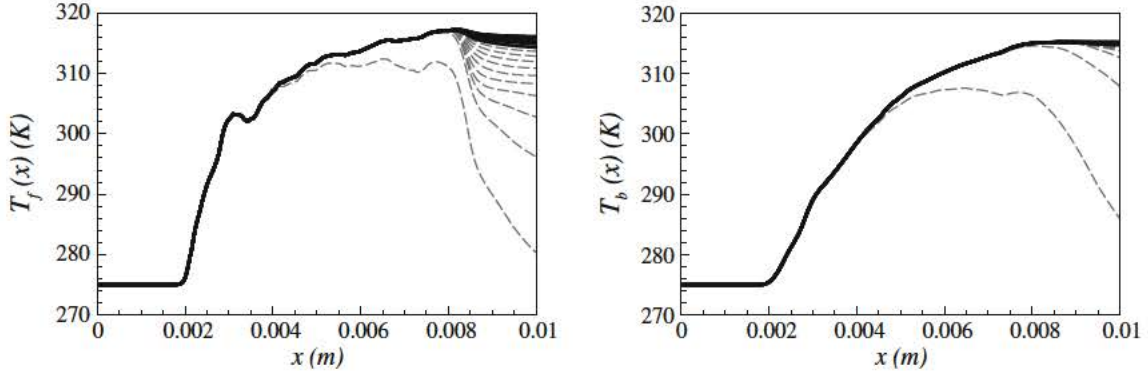
Fig. 12 Temperatures evolutions: T_f(x) (left) and T_b(x) (right) at Re = 50 and \phi = 0.4
