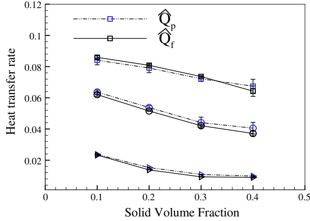
Fig. 13 Heat transfer rate for different particle concentration, at Re = 10 ▷, Re = 50 ○, and Re = 100 □
