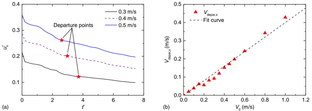
Fig. 6 (a) Variations of dimensionless horizontal velocity with time during jumping under different initial velocities. (b) Relationship between horizontal departure velocity and initial velocity of the moving droplet.
