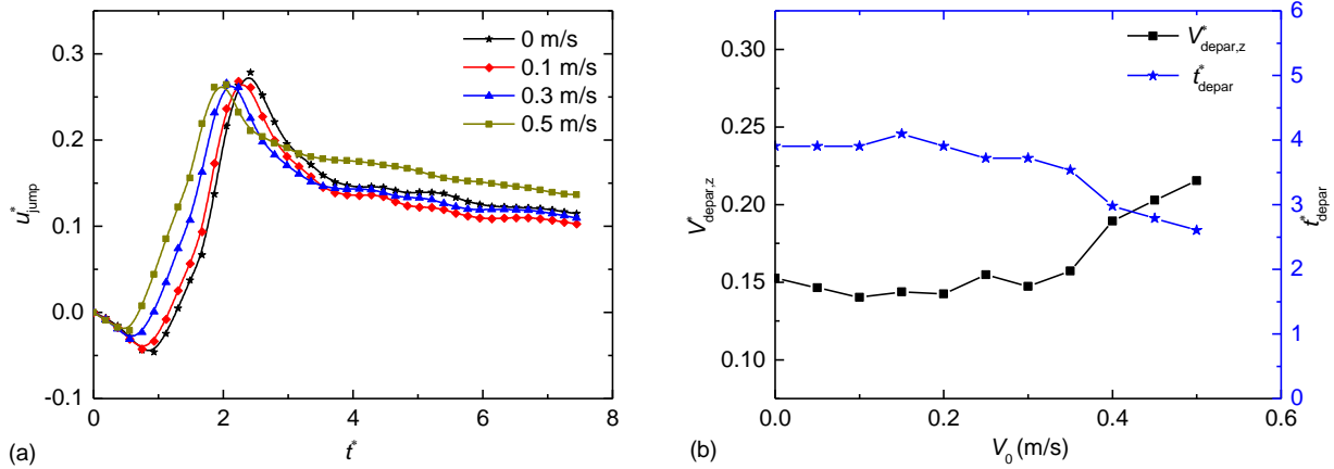
Fig.3 (a) Relationship between dimensionless jumping velocity and dimensionless time. The figure shows the tendency of the jumping speed under four different initial velocities: 0 m/s, 0.1 m/s, 0.3 m/s, 0.5 m/s, respectively. (b) Relationship between vertical departure velocity and departure time with respect to various initial velocities.
