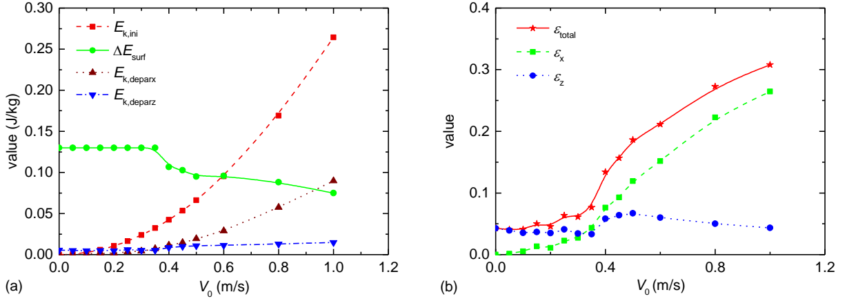
Fig. 7 Variations in (a) various energies and (b) energy conversion rates with different initial velocities at the droplet departure moment.
