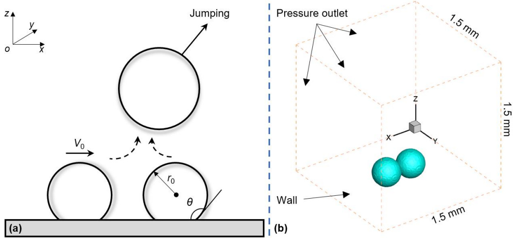
Fig. 1. (a) Schematic diagram of droplet jumping induced by coalescence of a moving droplet and a static one. The left droplet has a velocity which moves toward the stationary droplet and then they jump together after merge on the superhydrophobic surface. (b) 3D model of the simulation. At initial time, two droplets contact with each other. We set an initial velocity on the left droplet.
